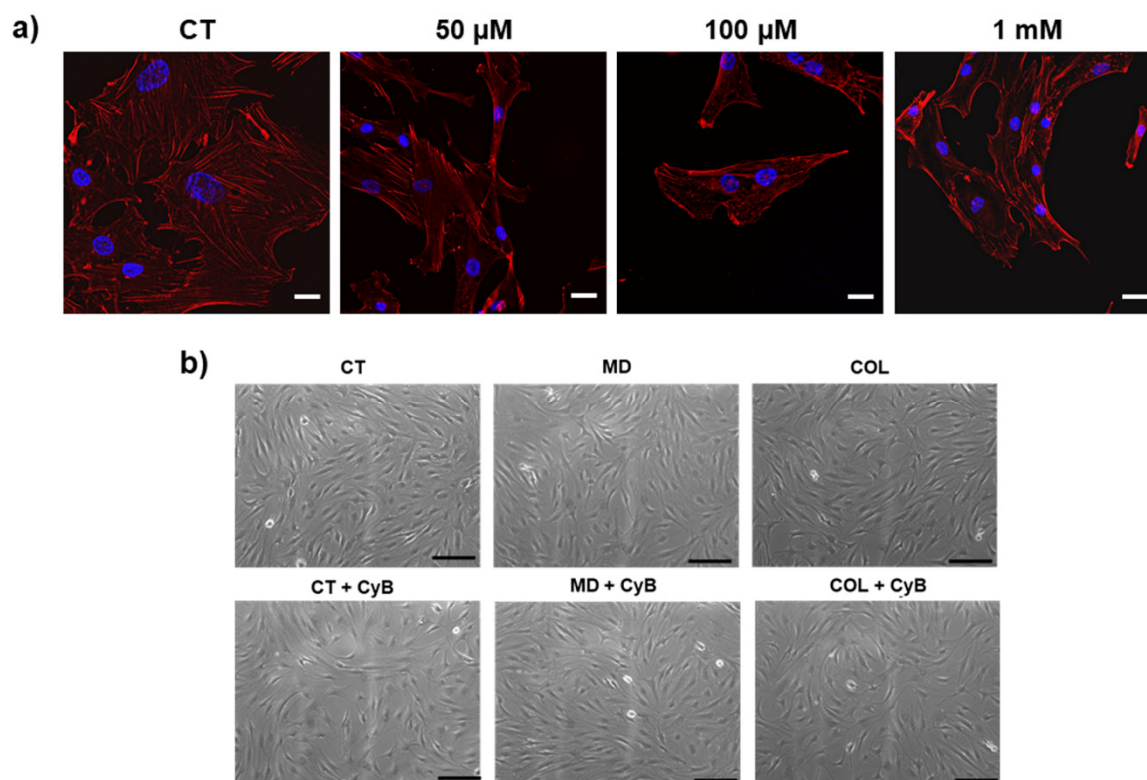
Figure 5. (a) Micrographs showing actin filaments detected by rodhamine-phalloidin by THUNDER in control cells (CT) and after administration of CyB at the indicated doses. After 50 µM CyB, actin filaments become shorter and more evident, indicating that the cytoskeleton is not preserved after CyB. (b) Representative phase contrast microscopy micrographs showing cell morphology of cells grown on MD and COL, compared to CT. After CyB, CT cells become less flattened and more rounded (Figure 4b). Scale bar 200 µm (a) and 20 µm (b).
